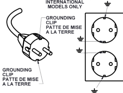
FIGURE C 230V NOMINAL / 50-60HZ 1-PHASE SHUKO CORD (TYPE F) INTERNATIONAL MODELS ONLY
